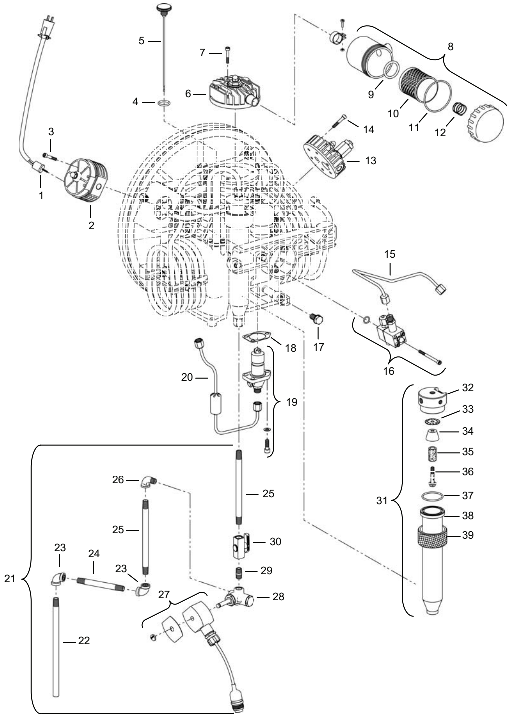
Figure 62. Air Compressor.
