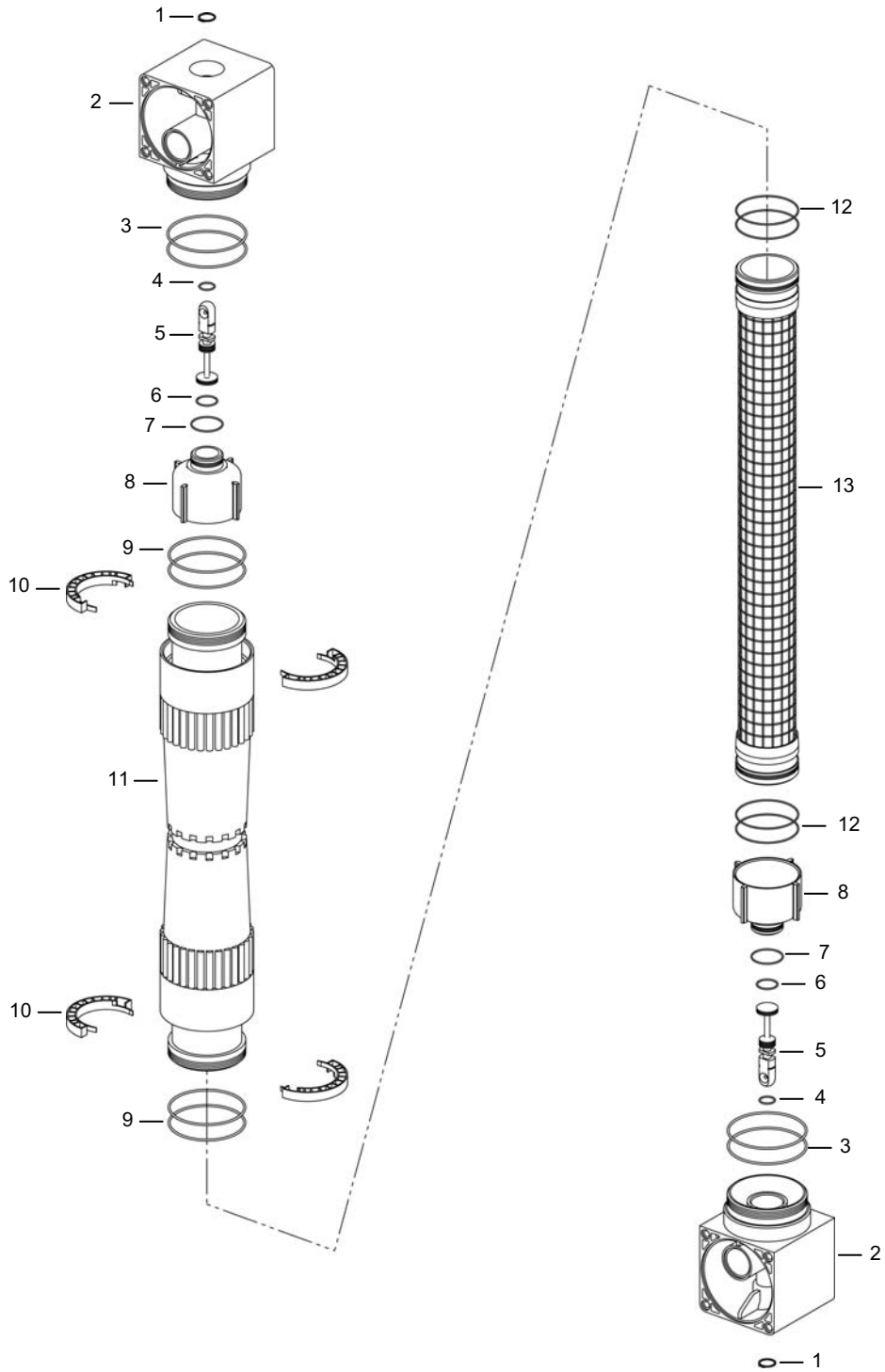
Figure 34. Filtration Module.
