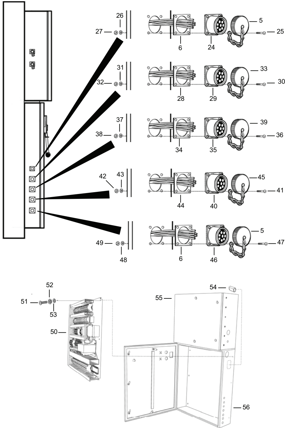
Figure 77. Power Distribution System (Sheet 2 of 3).
